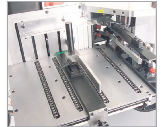
Magazine with chain feed
